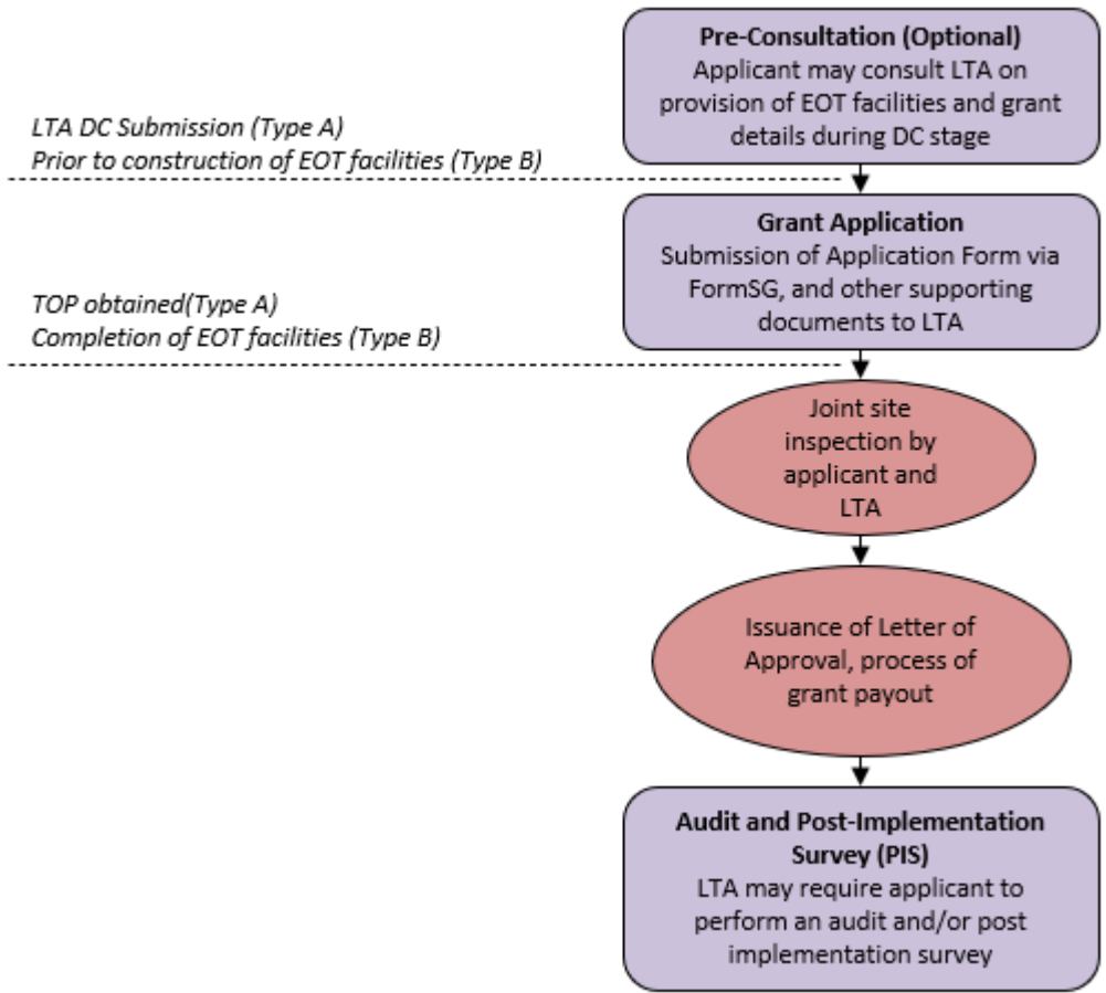
Figure 1: Application Flowchart
